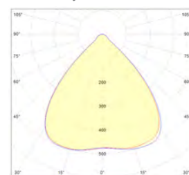
Photometry SWM
