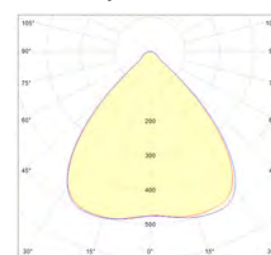
Photometry SWM
