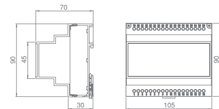
I0827 OnLED modulator 110V Modulador OnLED 110V
